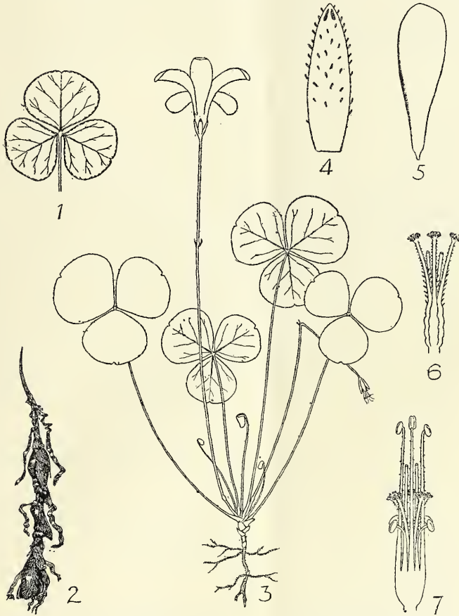
FIG. 5. Oxalis orbicularis , Salter. 1. Leaf (underside), natural size. 2. Bulb, natural size. 3. Plant, natural size. 4. Sepal \times 8 . 5. Petal \times 2 . 6. Gynaecium \times 6 . 7. Androecium \times 6 . (Salter 2323.) Del. T. M. Salter.
